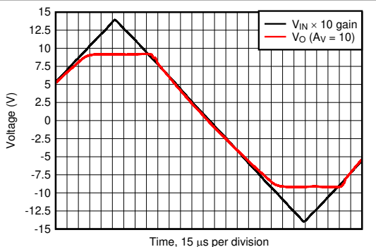
V_{IN} = 2.8\text{-V}_{PP} triangular waveform
